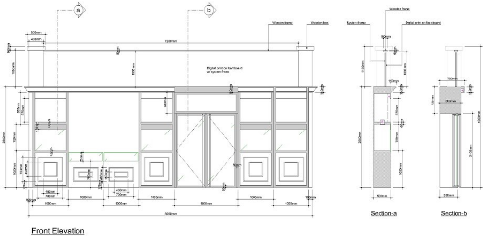
Front Elevation
