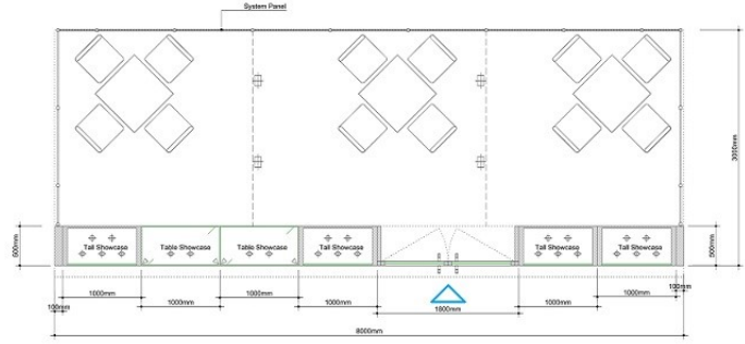
8M X 3M X 4M H (ONE SIDE OPEN BOOTH)
